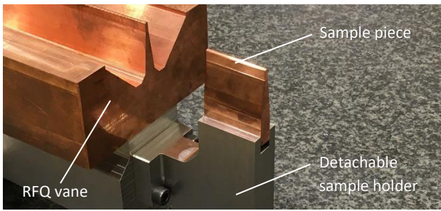
Figure 8. Sample piece installed for tool calibration purposes.
