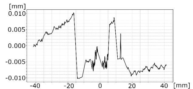
Figure 11. Deviation between nominal shape and measured transversal profile of a major vane.
