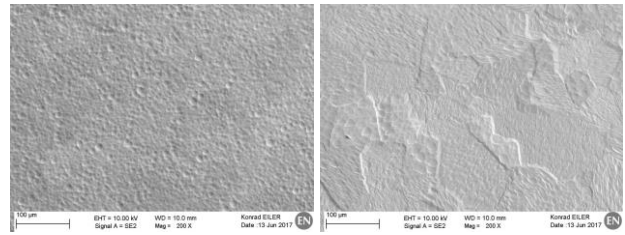
Figure 8. The SE overview of free-inclusions surface state after MMP & EP (left) and MMP & BCP (right).
