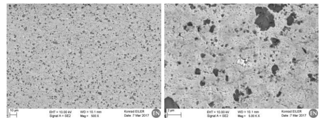
Figure 4. The SE overview of surface state after long treatment type Micro-tools_1 on Nb sample.
