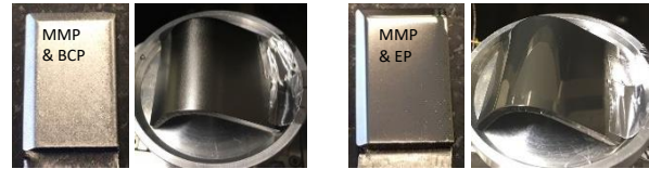
Figure 3. The comparison of the surface aspect of the niobium samples after MMP and BCP & EP.
