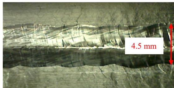
Figure 8: Weld root on the RF surface. Width of the root is 4.5 \text{ mm} .
