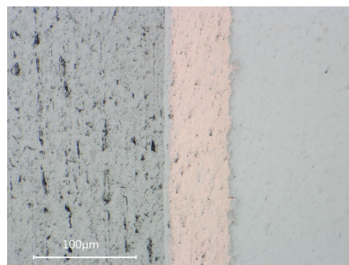
Figure 13: Vacuum brazing joint between a niobium tube (left), 1.4429 stainless steel flange (right) using copper as filler metal (centre).
